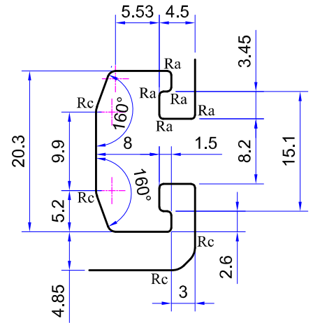
DETAIL - A (Typ.-4 Places)
