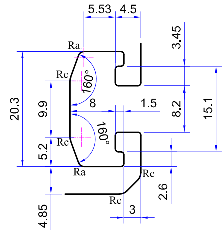
DETAIL - A (Typ.-5 Places)
